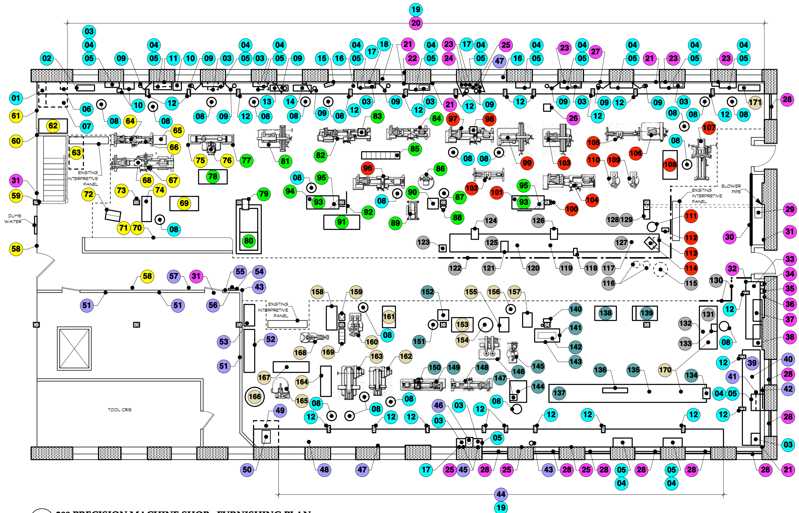
1 209 PRECISION MACHINE SHOP - FURNISHING PLAN SCALE: 1/8" = 1'-0"
